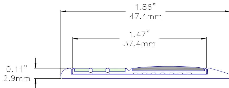
ECOGLO-PROFILE T3 SERIES WITH E20 SERIES INSERT
