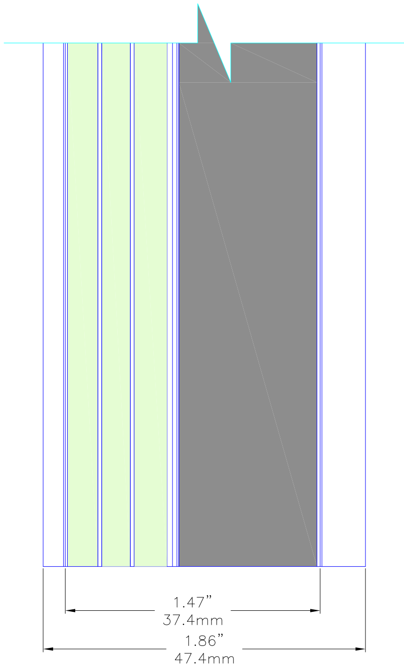
ECOGLO-TOP T3 SERIES WITH E20 SERIES INSERT
