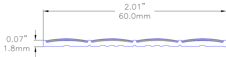
ECOGLO-PROFILE N10 SERIES NON-SLIP STRIP
