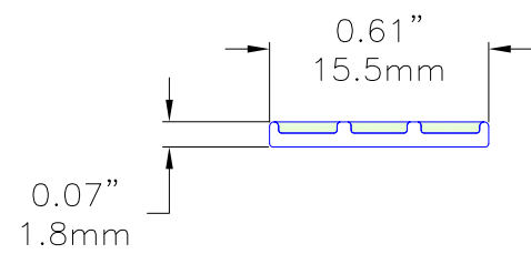
ECOGLO-PROFILE G SERIES GUIDANCE STRIP
