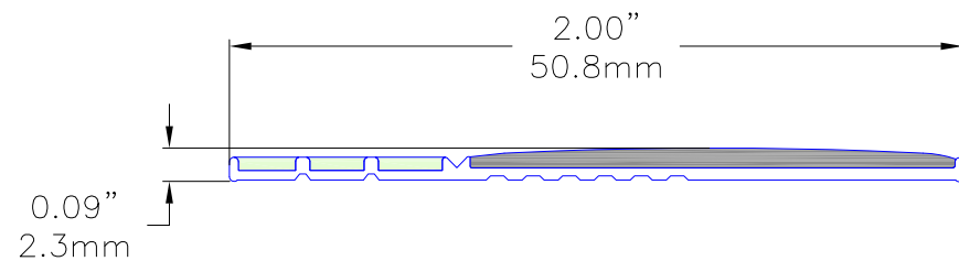
ECOGLO-PROFILE E30 SERIES CONTRAST STRIP
