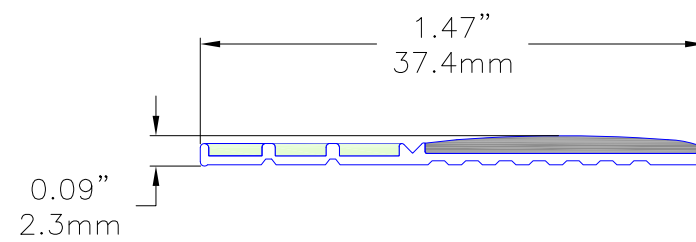
ECOGLO-PROFILE E20 SERIES NON-SLIP STRIP
